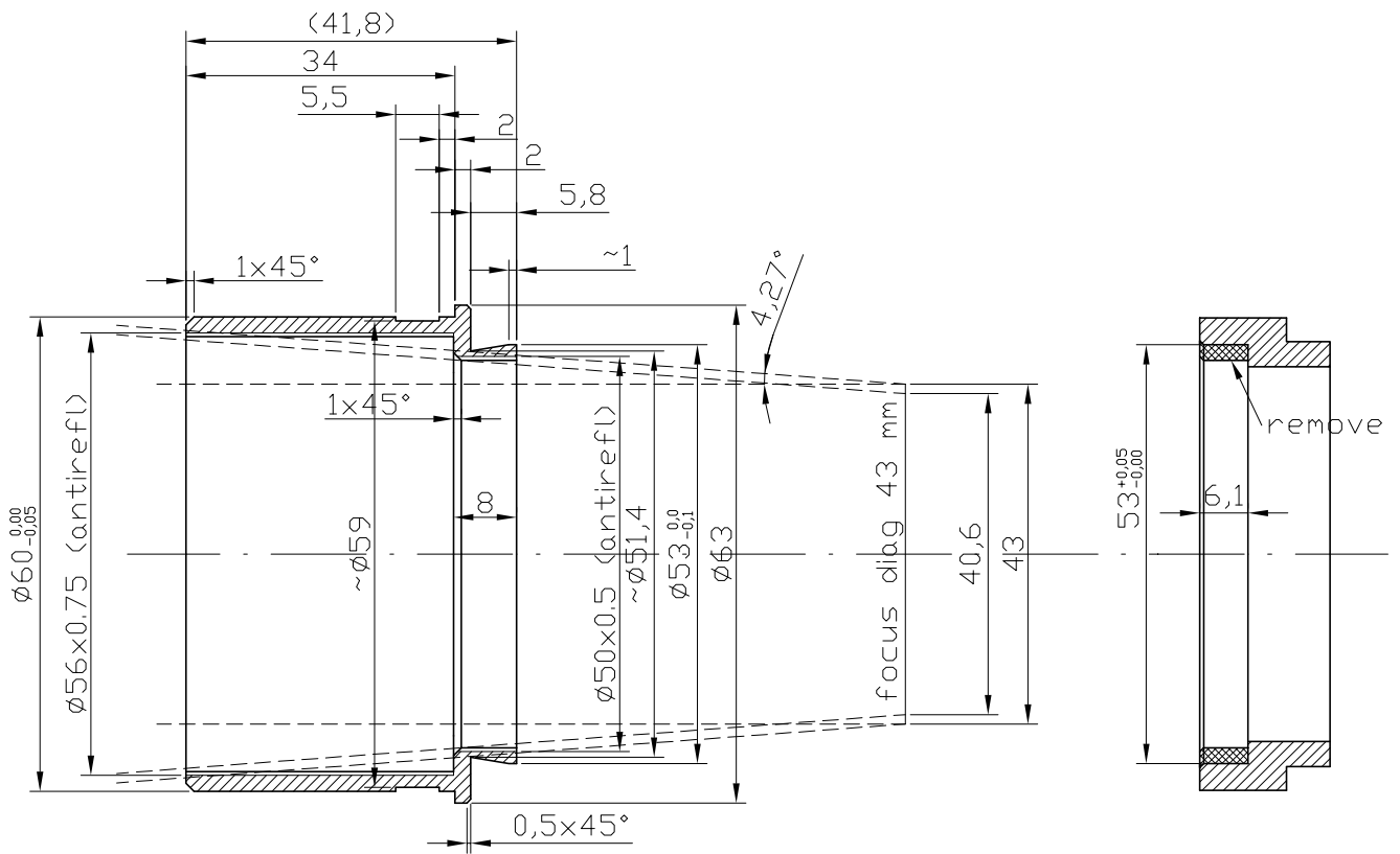
Modified Canon EOS T-adapter
